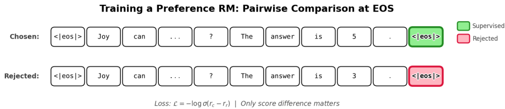
Figure 15: Training a preference reward model requires pairs of chosen and rejected completions. The model computes a scalar score for each completion from a sequence-level representation, often the end-of-sequence (EOS) token’s hidden state, and the contrastive loss depends only on the score difference between the two.
