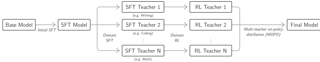
Figure 12: A schematic of specialist post-training with MOPD: shared SFT, domain-specific SFT and RL, then multi-teacher on-policy distillation into one (final) student.
