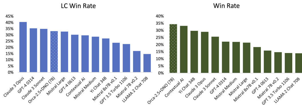
Figure 52: Results from the paper on Direct Nash Optimization (DNO) highlighting their small model outperforming the likes of GPT-4. Rosset et al. 2024. License CC-BY.
