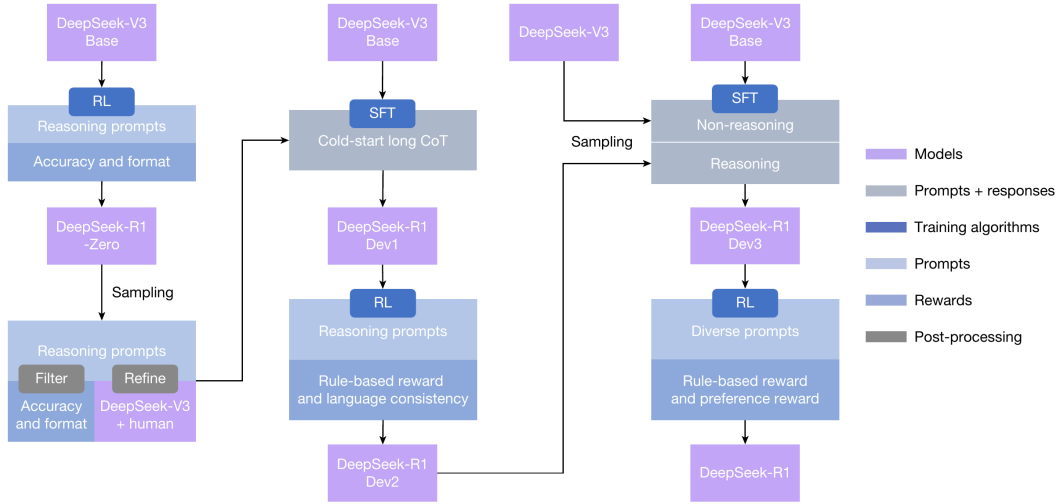
Figure 11: The multistage pipeline of DeepSeek-R1. From DeepSeek R1 paper in Nature , Fig. 2, under CC BY 4.0 [15].
