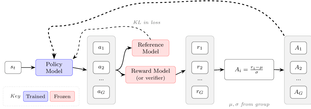
Figure 25: GRPO architecture. Advantages are normalized relative to the group mean and standard deviation. The KL penalty is applied directly in the loss rather than shaping the reward.
