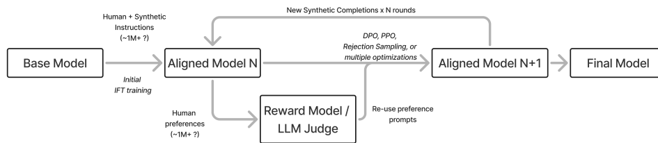
Figure 9: A rendition of modern post-training with many rounds.
