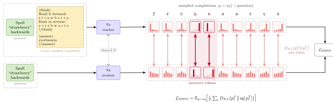
Figure 41: On-policy self-distillation (OPSD) on a string-reversal task. One policy \pi_\theta is forwarded twice over the same student-sampled completion y : a teacher pass conditioned on the question plus a correct sibling demonstration (yellow), and a student pass conditioned on the question only (green). The per-token reverse KL between the two passes, with a stop-gradient on the teacher, pulls the question-only policy toward its demonstration-conditioned self; highlighted columns are the incorrectly sampled tokens where the distributions diverge most.
