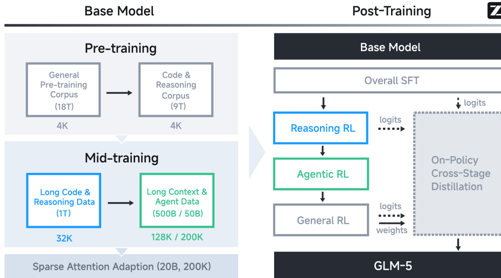
Figure 13: Overall training pipeline of GLM-5. From the GLM-5 Team’s paper, Fig. 5, under CC BY 4.0 [68].
