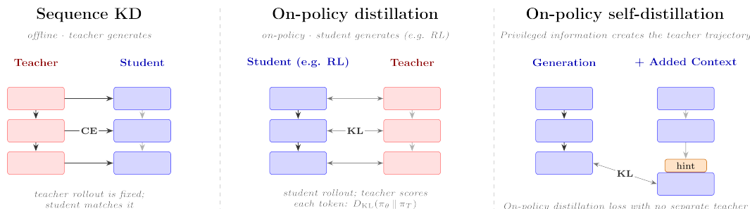
Figure 40: Three distillation regimes, compared by where the rollout comes from and how supervision flows. Sequence KD (left): the teacher generates an output offline and the student is trained to match it with a cross-entropy (CE) loss. On-policy distillation (OPD) (center): the student generates the rollout on-policy (e.g. within a RL framework) and a separate teacher scores each visited token, training the student with a per-token KL divergence (KL). On-policy self-distillation (OPSD) (right): one model plays both roles – privileged information (a hint) added to the context creates a teacher trajectory, and the no-hint generation is distilled toward it with a KL loss, with no separate teacher model.
